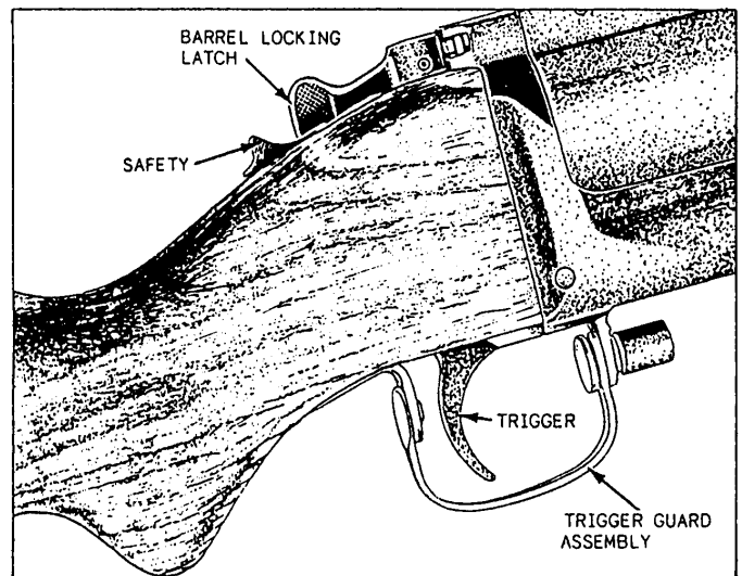
Figure 8-40.-M79 Grenade launcher controls.
