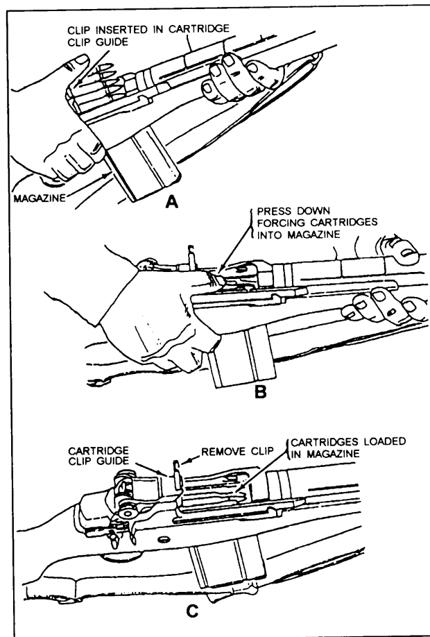
Figure 8-14.—Loading the magazine through the cartridge clip guide.
