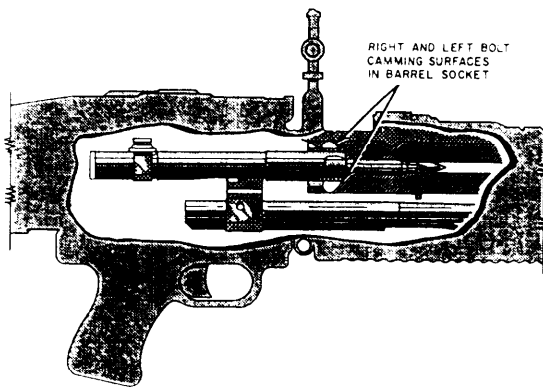
Figure 8-34.-Weapon locked, ready to fire.
