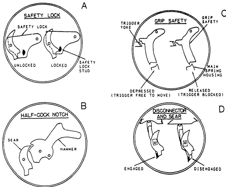
Figure 8-6.—Safeties on the .45-cal. pistol.
