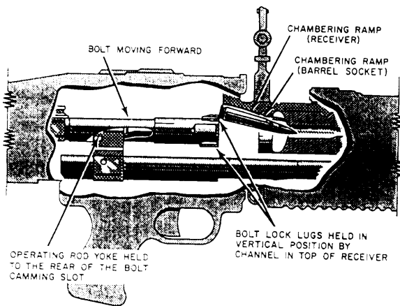
Figure 8-33.-Chambering.
