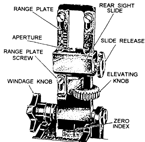
Figure 8-30.-M60 rear sight.
