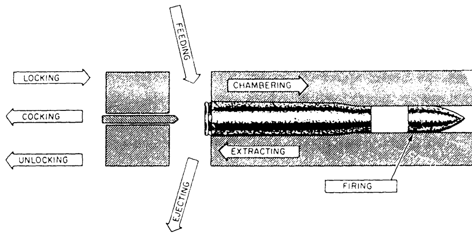
Figure 8-1.—The small arms cycle of operation.
