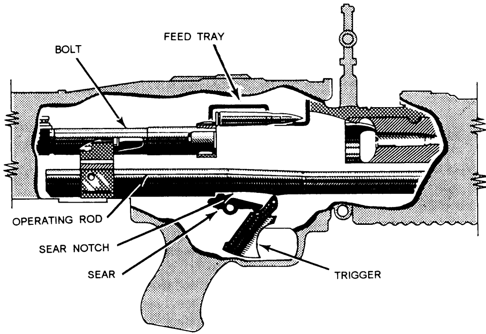
Figure 8-31.-Sear disengaging from sear notch.
