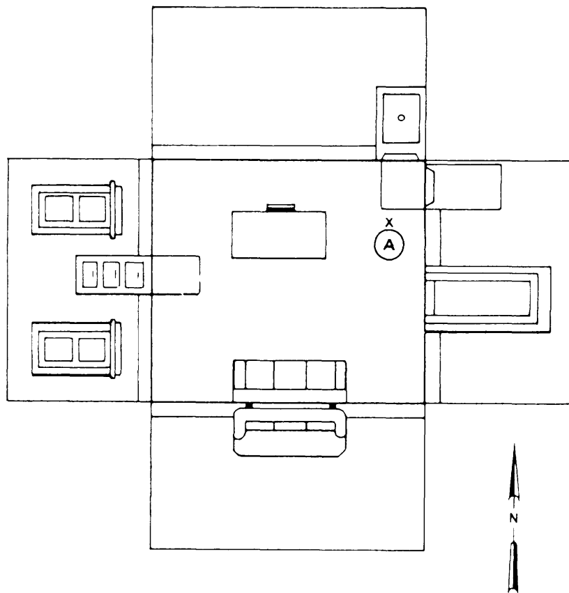
Figure 16-18.-Projection drawing.
